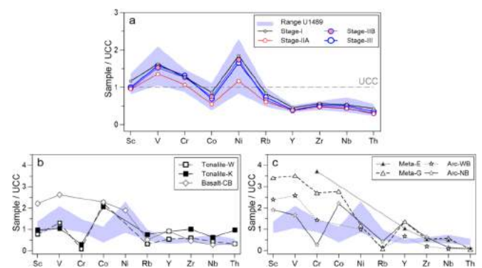
Fig. 4. Trace-element distribution pattern of IODP Site U1489 sediments. (a) Sediment samples of Site U1489, showing the distribution range of all samples (light blue shading; also in b–c) and the average values for the evolutionary stages (lines with symbols). (b) Tonalites (squares; Holm et al., 2015) from Wamum (Tonalite-W) and Kainantu (Tonalite-K), and basalts (diamonds) from the Cloudy Bay (Basalt-CB; Holm and Poke, 2018). (c) Metamorphic rocks (triangles) from Emo (Meta-E; Zirakparvar et al., 2013) and Goropu (Meta-G; Smith, 2013), and arc volcanic rocks (stars) from New Britain (Arc-NB; Holm et al., 2013) and Western Bismarck arc (Arc-WB; Woodhead et al., 2010). Note that the transition elements Sc, V, Co, Cr, and Ni are typically enriched in mafic igneous rocks, whereas Rb, Y, Zr, Nb, and Th are more concentrated in felsic rocks (c.f. McLennan et al., 1993). All trace elements are normalized to mean values of the upper continental crust (UCC; Rudnick and Gao, 2003). See Fig. 1b for the locations of the potential source rocks. (For interpretation of the references to colour in this figure legend, the reader is referred to the web version of this article.)
